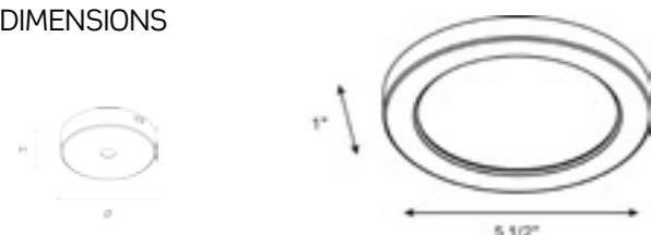
CANOPY: Ø: 3 15/16"xH: 7/8"
