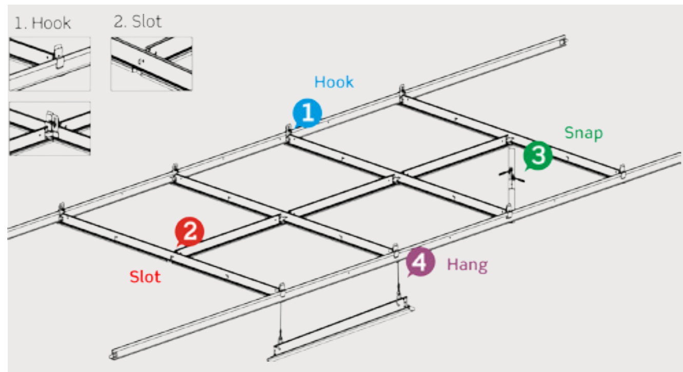
Mounting Layout Configuration as shown in photo
